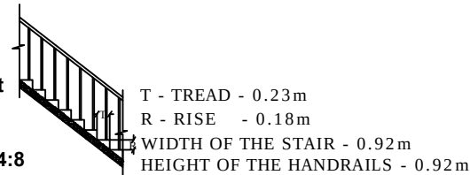
STAIRCASE DETAILS
