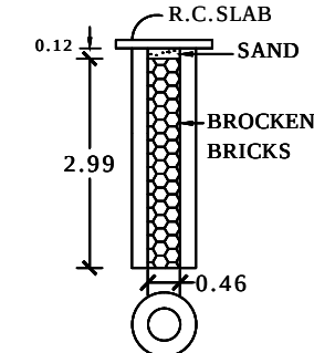
PERCOLATION PIT
