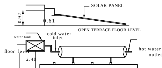
Details of solar water heating system
