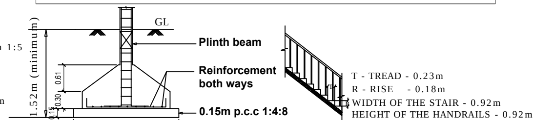
STAIRCASE DETAILS
