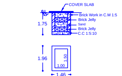
PLAN & SECTIONAL ELEVATION OF RAIN WATER HARVESTING
