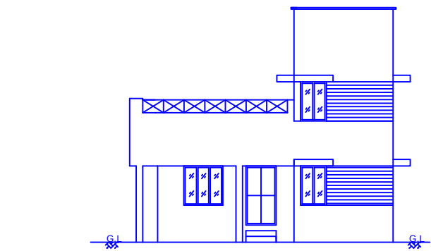
FRONT ELEVATION
