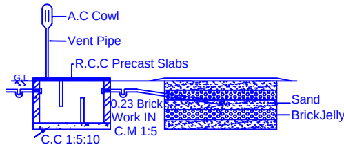
SECTION ON"BB" 'U' TROP MODEL S.T.ADOPTED )
