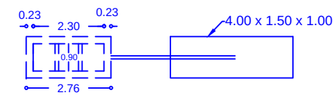
PLAN OF SEPTIC TANK & DISPERSION TRENCH
