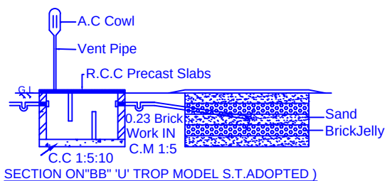
SECTION ON "BB" 'U' TROP MODEL S.T.ADOPTED )
