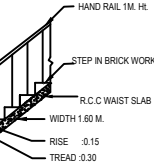
STAIR DETAIL
