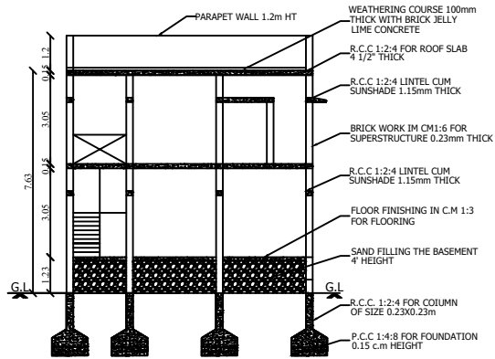
SECTION ON-AB
