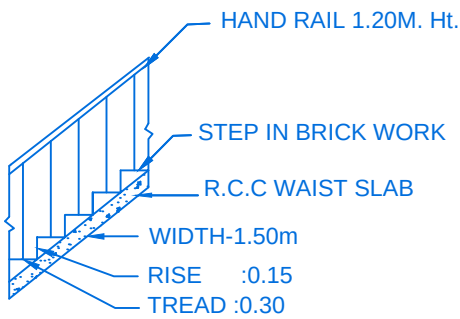
STAIR DETAIL
