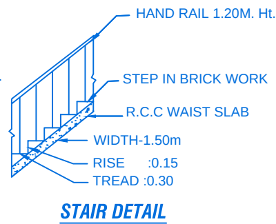
STAIR DETAIL
