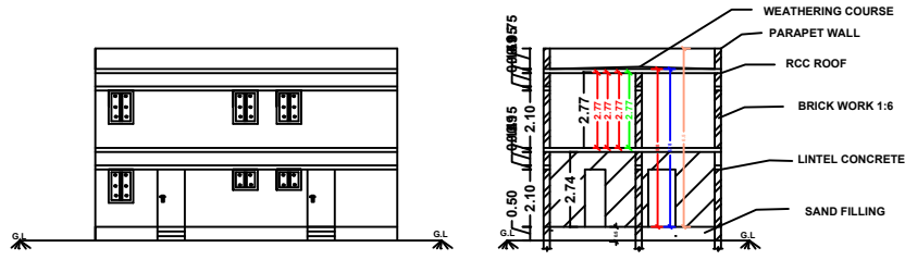
SECTION AB
