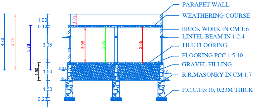
SECTION ON "V-B"
