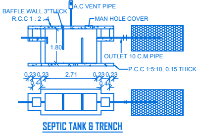
SEPTIC TANK & TRENCH
