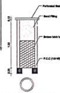
RAIN WATER COLLECTION WELL
