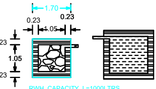
DETAILS OF FILTER BED & WELL
