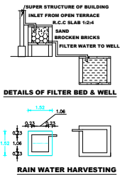
RAIN WATER HARVESTING
