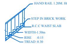
STAIR DETAIL
