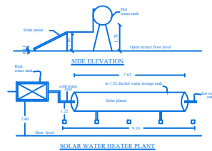
SOLAR WATER HEATER PLANT
