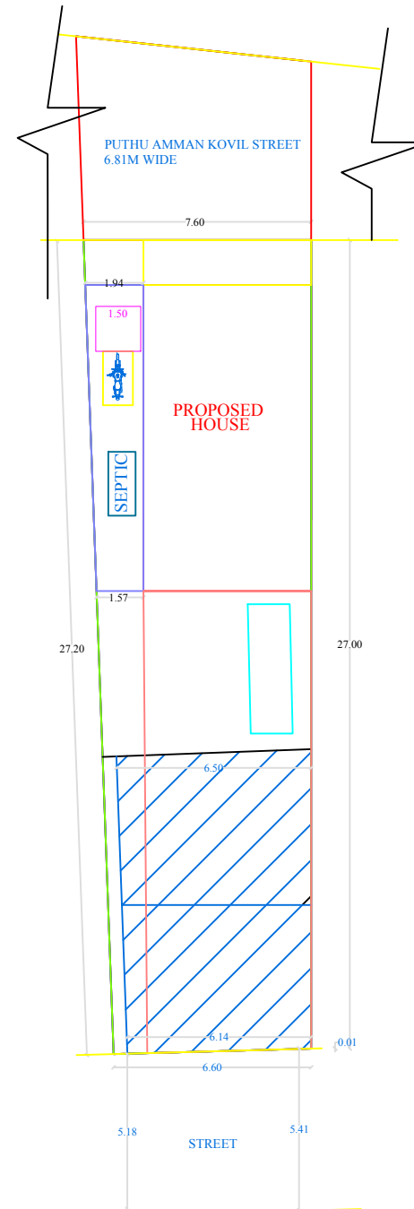
TOPO PLAN (Scale 1 : 5000)
