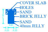
SECTION OF RAIN WATER COLLECTION TANK
