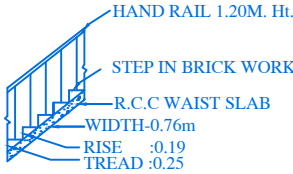
STAIR DETAIL
