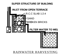
RAINWATER HARVESTING
