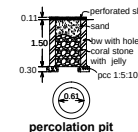
percolation pit
