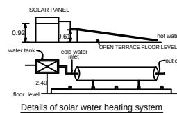
Details of solar water heating system
