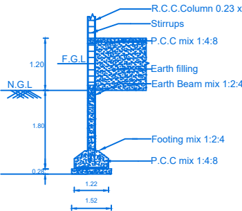
COLUMN DETAILS
