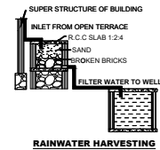
RAINWATER HARVESTING
