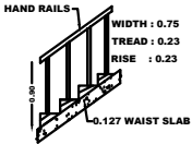
STAIRCASE DETAILS:-
