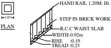
STAIR DETAIL
