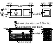
Details of septic tank & trench
