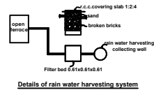
Details of rain water harvesting system
