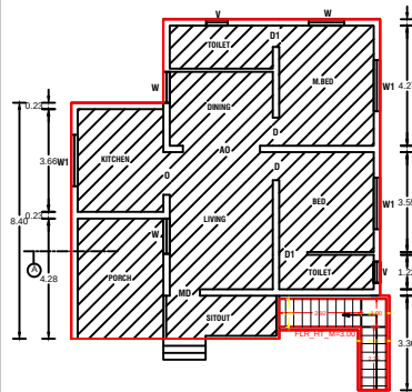
EXG.GROUND FLOOR PLAN
