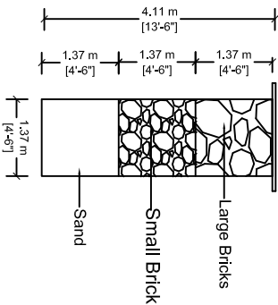
SECTION OF RAIN WATER COLLECTION PITS (NTS)
