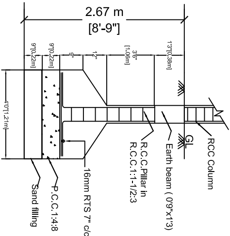
FOUNDATION DETAILS
