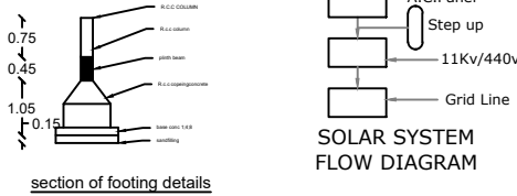
section of footing details
