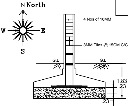
RCC COLUMN DETAILS
