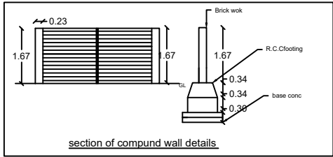
section of compound wall details
