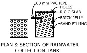
PLAN & SECTION OF RAINWATER COLLECTION TANK
