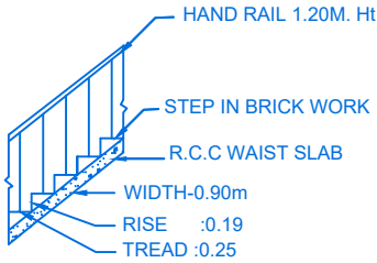
STAIR DETAIL (EXG.)
