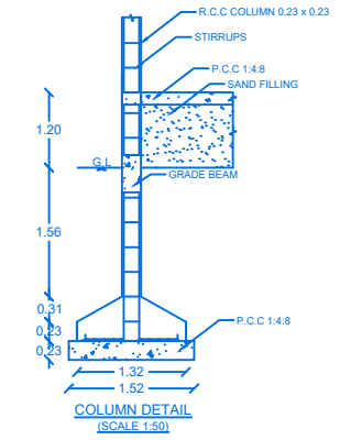
COLUMN DETAIL (SCALE 1:50)
