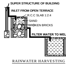
RAINWATER HARVESTING
