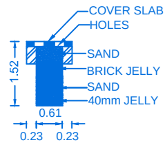
SECTION OF RAIN WATER COLLECTION TANK
