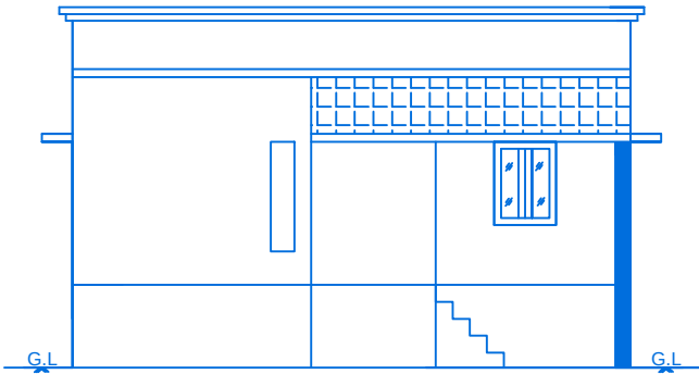
FRONT ELEVATION
