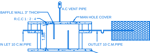
SEPTIC TANK AND TRENCH & U TRAP ADOPTED
