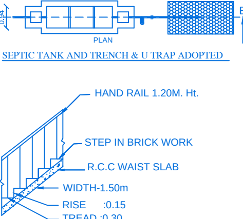
STAIR DETAIL
