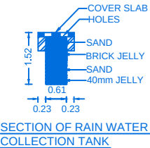
SECTION OF RAIN WATER COLLECTION TANK
