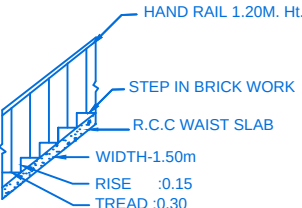
STAIR DETAIL
