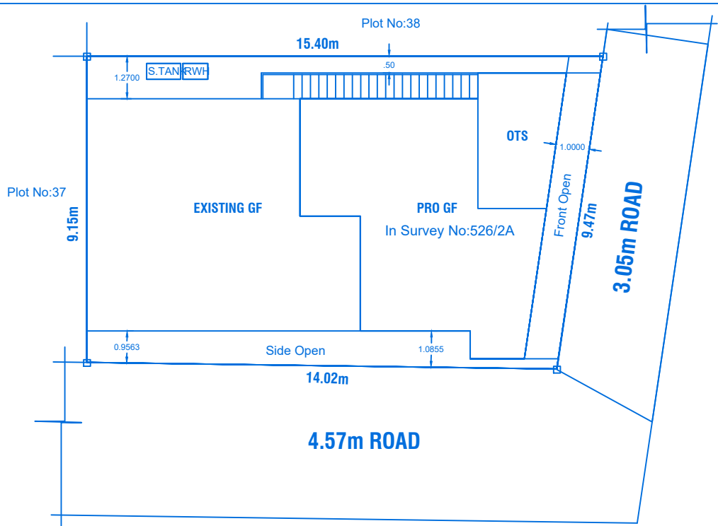
SITE PLAN
