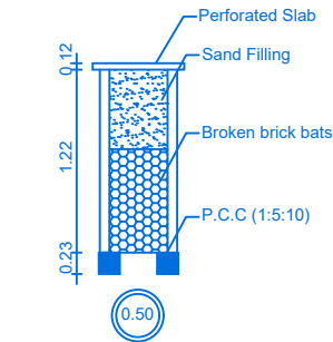
RAIN WATER COLLECTION WELL
