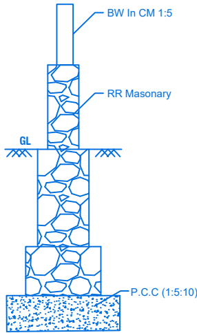
DETAILS OF RR MASONRY
