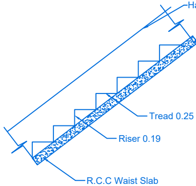
STAIR DETAILS
