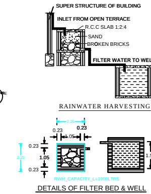
DETAILS OF FILTER BED & WELL
