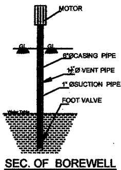
SEC. OF BOREWELL
