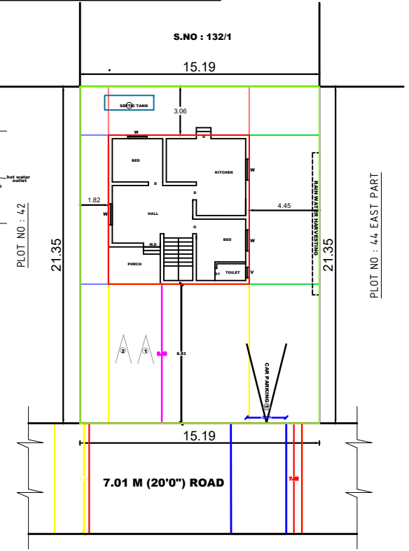
TOPO SKETCH
