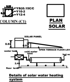
Details of solar water heating system
