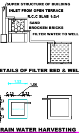
RAIN WATER HARVESTING
