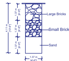
SECTION OF RAIN WATER COLLECTION PITS (NTS)
