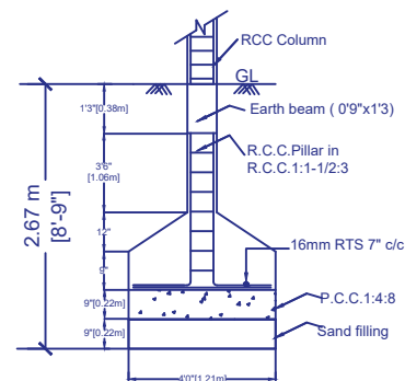
FOUNDATION DETAILS
