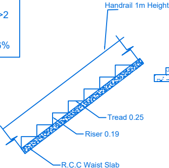
STAIR DETAILS
