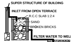
RAINWATER HARVESTING
