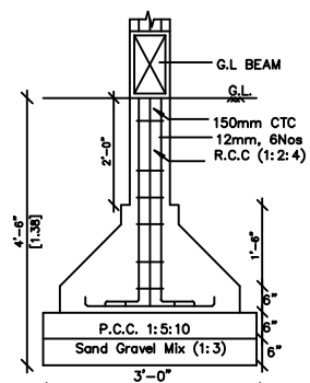
R.C.C. COLUMN FOOTING DETAILS
