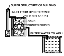
RAINWATER HARVESTING
