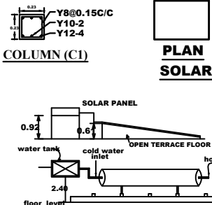
Details of solar water heating system
