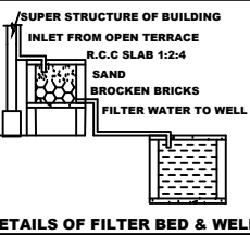
DETAILS OF FILTER BED & WELL
