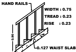
STAIRCASE DETAILS:-
