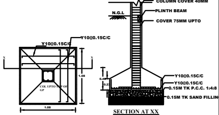
SECTION AT XX
