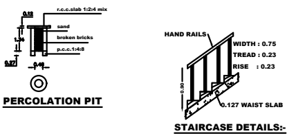
STAIRCASE DETAILS:-
