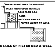
DETAILS OF FILTER BED & WELL
