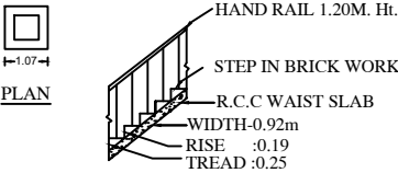
STAIR DETAIL
