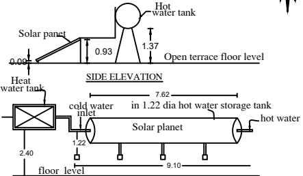
SOLAR WATER HEATER PLANT
