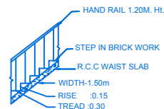
STAIR DETAIL
