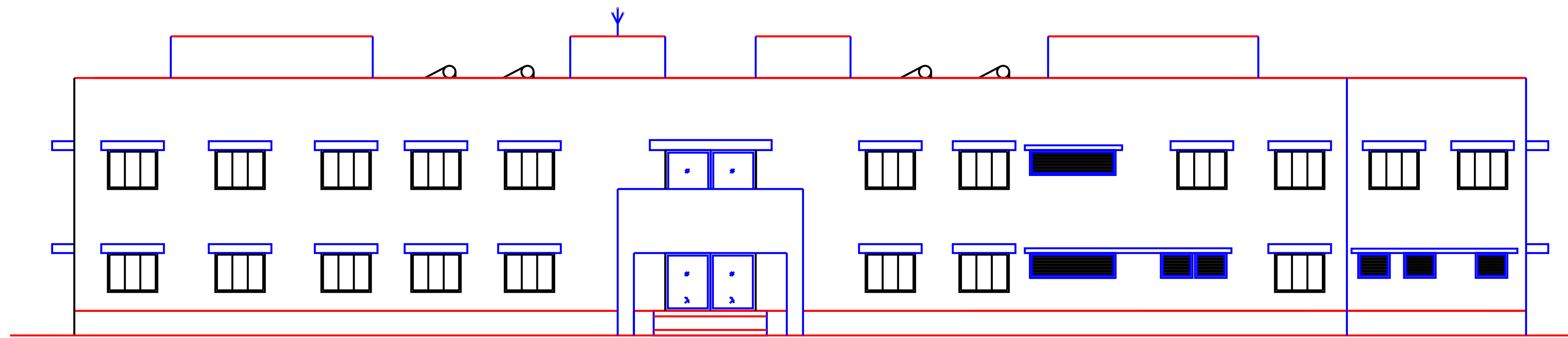
FRONT ELEVATION
