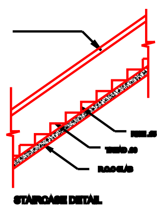
STAIRCASE DETAIL
