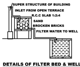
DETAILS OF FILTER BED & WELL
