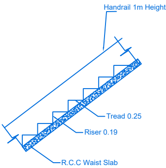
STAIR DETAILS
