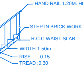
STAIR DETAIL
