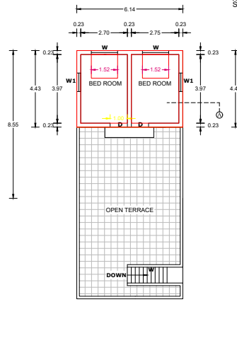
PRO.SECOND FLOOR PLAN
