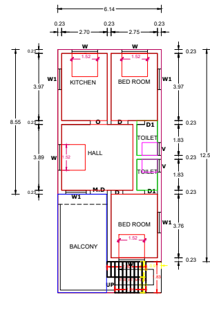
PRO.FIRST FLOOR PLAN
