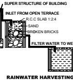
RAINWATER HARVESTING
