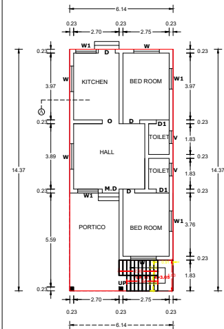
EXG.GROUND FLOOR PLAN
