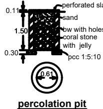
PERCOLATION PIT
