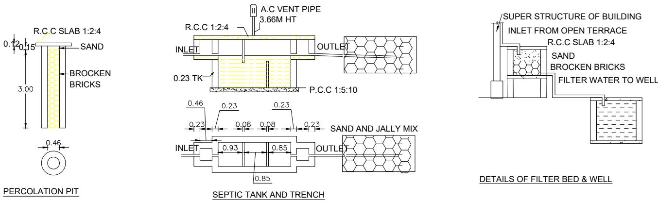
SEPTIC TANK AND TRENCH
