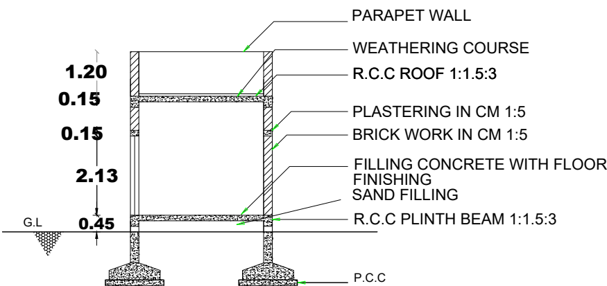
CROSS SECTION ON AA'
