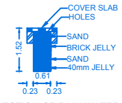
SECTION OF RAIN WATER COLLECTION TANK
