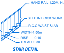
STAIR DETAIL
