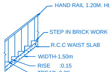
STAIR DETAIL
