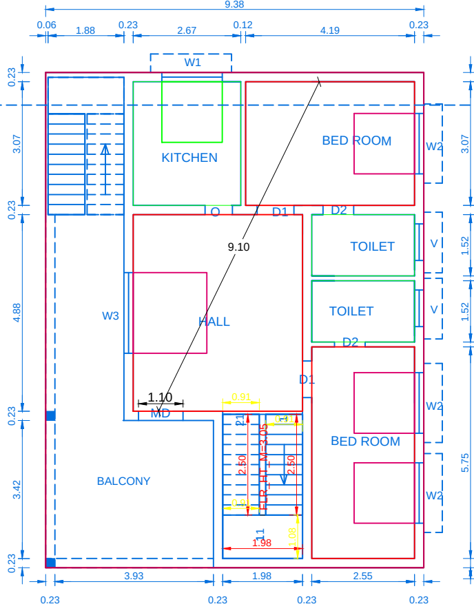
PROP.FIRST FLOOR PLAN
